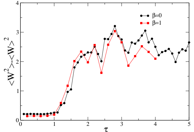
FIG. 11: Variance of the work distribution for the XX quantum chain with N = 8 spins at \beta = 0 and \beta = 1 for h_o = 1/2 as a function of the field period \tau .
