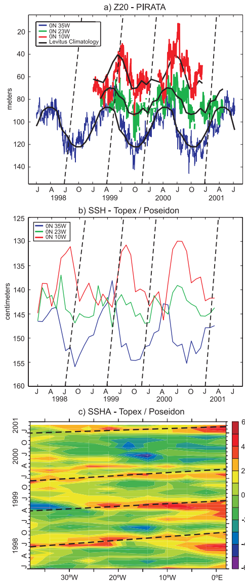
Figure 2. (a) Daily time series of Z20 provided by the PIRATA data at 0°N–35°W (blue), 0°N–23°W (green) and 0°N–10°W (red) superimposed to the monthly climatic values deduced from L82 (black lines); (b) Monthly times series of SSH as in (a) but from the T/P altimetry data set; (c) time-longitude diagram of SSH anomaly (humps in blue, hollows in red) along the equator during January 1998 to July 2001, as provided by the T/P altimetry data set. Eastward propagating events are identified in (c) by four dashed lines, also represented on (a) and (b).
