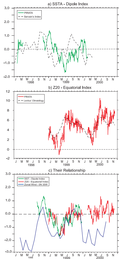
Figure 1. (a) Daily time series of the PIRATA SST dipole index (green line) superimposed to the Servain's [1991] dipole index (black dashed line); (b) Daily time series of the PIRATA Z20 equatorial slope (red line) superimposed to the monthly slope deduced from L82 climatology (black dashed line); (c) PIRATA SST dipole index (green line) and Z20 equatorial index (red line), superimposed to the zonal wind ( W_x ) monthly anomaly at 0^{\circ}\text{N} – 35^{\circ}\text{W} (blue line) deduced SL90 data. The time axis on (c) is related to the Z20 index; the SST dipole index is shifted backward by 2-month, whereas W_x is shifted forward by 2-month.
