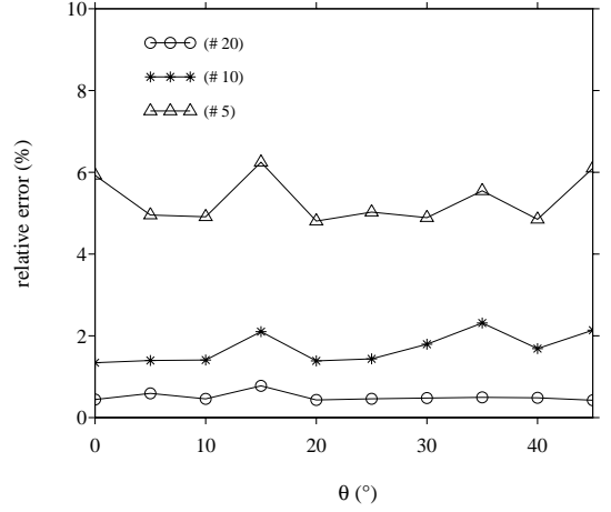
Figure 8. Test 2: parametric study of the relative error in terms of the boundary's angle \theta , with various discretizations. The number after # denotes the number of grid nodes per minimal S-wavelength.
