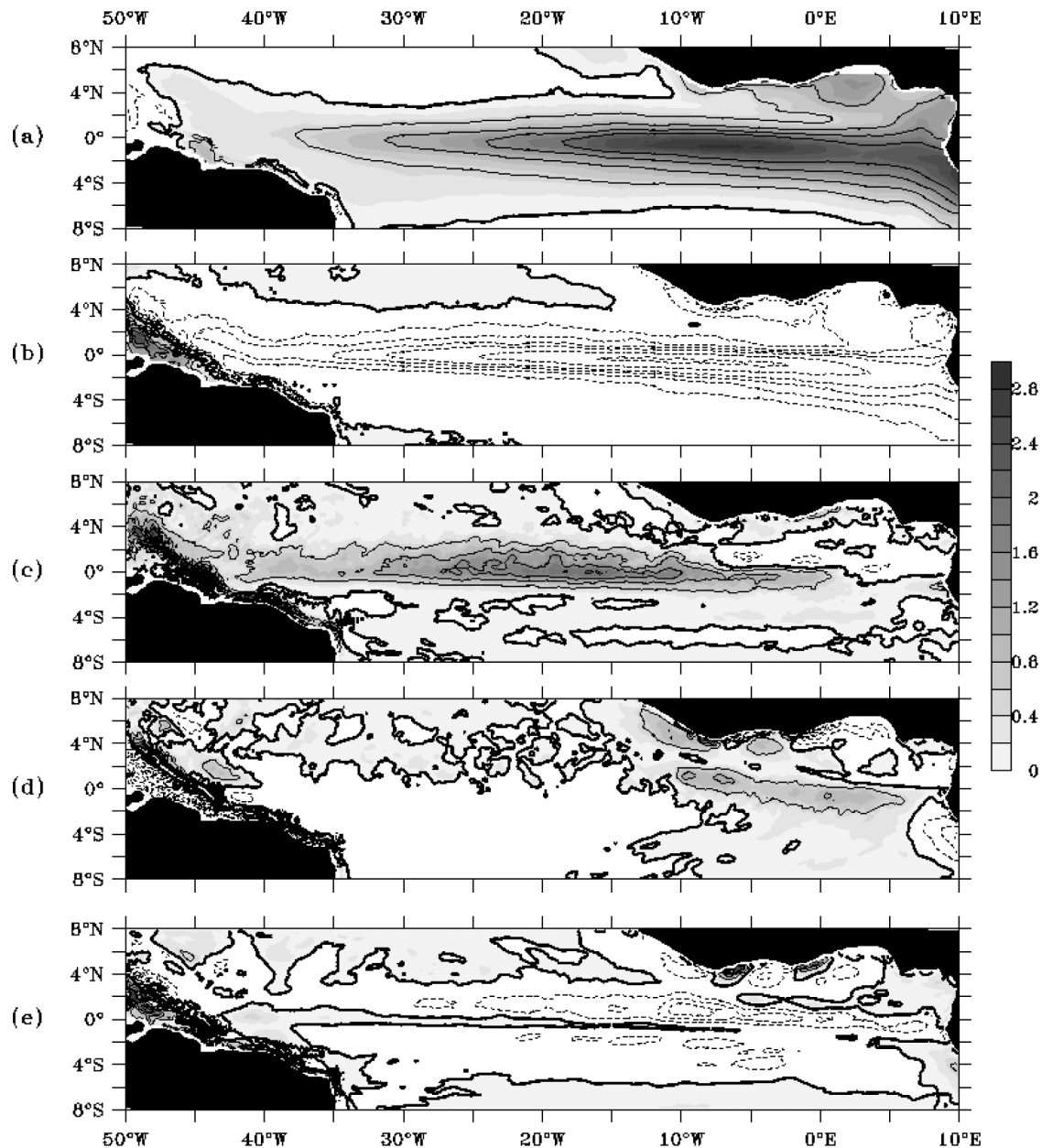
Figure 5. Longitude-latitude plots of the 1977–2000 time average of various contributors to the mixed layer temperature: (a) atmospheric forcing, (b) tendencies due to vertical exchanges with the subsurface ocean (sum of vertical advection, vertical diffusion at the base of the mixed layer, and entrainment), (c) eddies (high-frequency horizontal advection plus lateral diffusion), (d) zonal advection by low-frequency currents, (e) meridional advection by low-frequency currents (contours every 0.5^{\circ}\text{C month}^{-1} between -2^{\circ}\text{C month}^{-1} and 2^{\circ}\text{C month}^{-1} and every 1^{\circ}\text{C month}^{-1} after; the thick line is zero; and dashed contours represent negative values).
