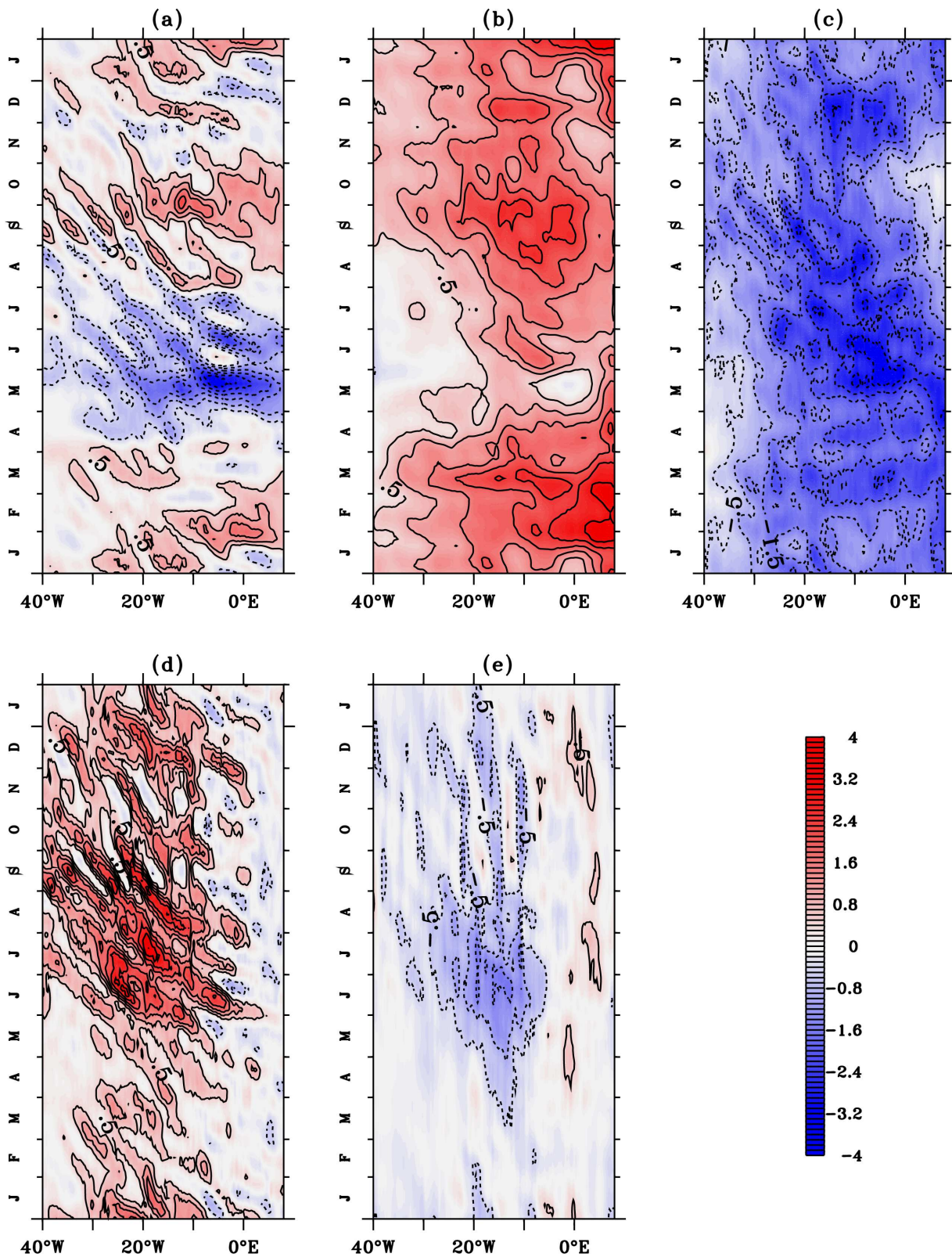
Figure 8. Longitude-time plots along the equator ( 2^{\circ}\text{N} – 2^{\circ}\text{S} average) of 1997–2000 mean seasonal cycles of (a) heat storage, (b) atmospheric forcing, (c) tendencies due to vertical exchanges with the subsurface ocean (sum of vertical advection, vertical diffusion at the base of the mixed layer, and entrainment), (d) eddies (high-frequency horizontal advection plus lateral diffusion), and (e) zonal and meridional advective tendencies by low-frequency currents (contours every 0.5^{\circ}\text{C month}^{-1} between -2^{\circ}\text{C month}^{-1} and 2^{\circ}\text{C month}^{-1} and every 1^{\circ}\text{C month}^{-1} after; the thick line is zero). All the trends are smoothed with a 25-day Hanning filter.
