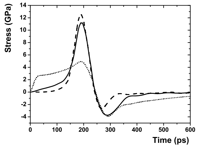
FIG. 3: Time evolution of the stress in copper at 1 \mu\text{m} depth resulting from a 170 fs, 10 J/cm 2 laser pulse. Standard conditions : \gamma = \gamma_0 and K_e = K_{e_0} (solid line), \gamma = 5\gamma_0 (dashed line), K_e = 10K_{e_0} (dotted line).
