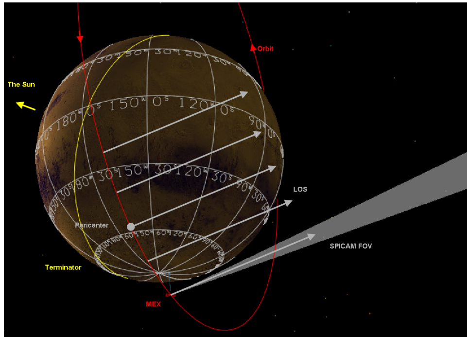
Figure 7. Geometry of grazing limb observations, which allows us to maximize the time spent to observe the limb. The spacecraft is oriented with the +Z axis (SPICAM LOS) fixed inertially, scanning the limb twice. In this case, the LOS was perpendicular to the velocity vector at pericenter, for an optimum vertical resolution at the limb.
