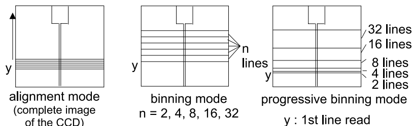
Figure 4. The various modes of SPICAM UV CCD reading. (left) A complete image of the CCD is obtained by groups of 5 lines (with 1 line overlap), in order to find the spectrum of the star (alignment mode, used very rarely). (center) The binning mode is the most often used, when 5 bins of 2, or 4, 8, 16, 32 lines are grouped together. The first line may be selected anywhere. (right) The progressive binning mode is used for higher dynamics: 32 lines for a weak signal, 2 lines for a strong signal. This mode was used at the beginning of MEX mission to explore the actual intensities observed.
