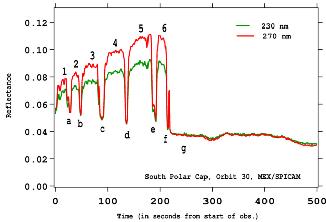
Figure 22. Nadir UV reflectance (radiance/cos SZA) at 230 nm and 270 nm along track over the South Polar cap and farther north (on the left). Letters a, b, c, d, e, f, and g indicate regions of low reflectance, both in UV SPICAM data and in the Viking image of the polar cap. The UV albedo is much larger on lobes 1, 2, 3, 4, 5, and 6 of ice identified on the Viking images than outside the cap (region beginning at letter g). While the reflectance at 230 and 270 nm is equal outside the cap and between the lobes, it is lower at 230 than at 270 nm on the lobes, typical of the known signature of ices.
