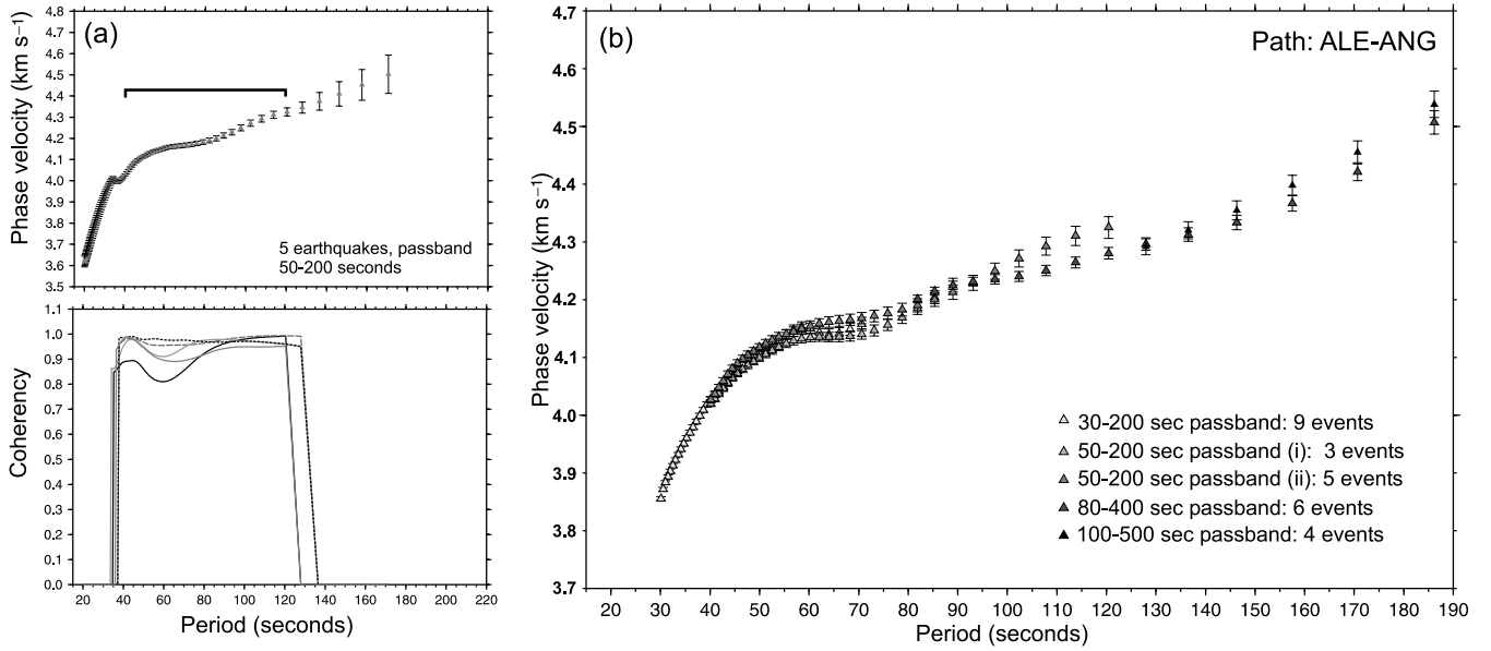
Figure 5. (a) Example of dispersion curve computed for five earthquakes in the 50–200 s passband, for path ALE–ANG. Top: dispersion curve with error bars. The horizontal bar indicates where the results are well resolved and reliable. Bottom: waveform coherencies for the five earthquake pairs used in the analysis. (b) Composite dispersion curve for path ALE–ANG, composed of reliable results from several different passbands using several seismogram pairs in each case.
