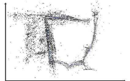
Figure 5. The long urban sequence a) left: some frames from the sequence, b) right: a map of the city with the trajectory in blue, the reconstruction result (trajectory and 18,403 3D points).
