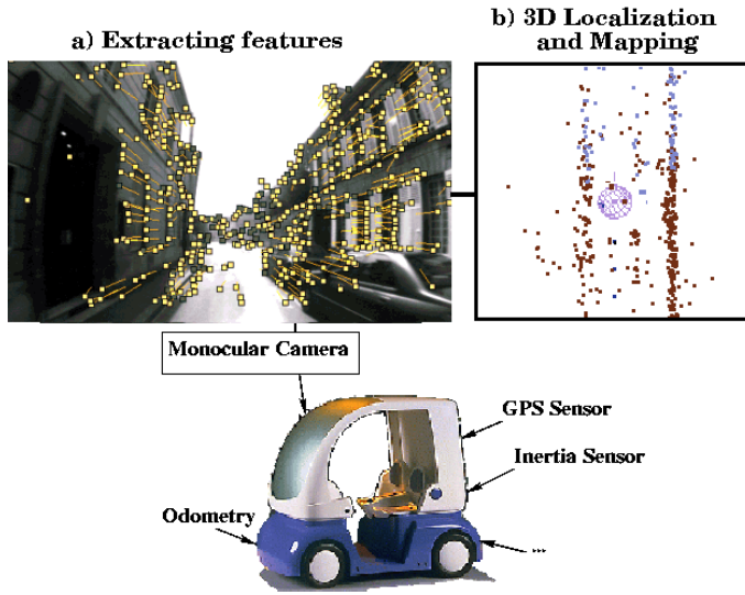
Figure 1. Monocular Vision among other sensors. a) An example of image and points tracks. b) Top view of the real time localization. We can see 3D reconstructed points and the ellipsoid of confidence for the current camera pose.
