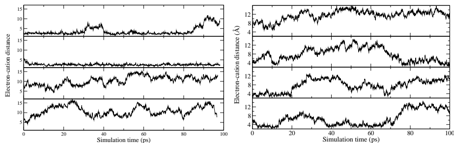
Figure 8: Electron-cation distance as a function of simulation time during unconstrained simulations of K^+ (left panel) and Li^+ (right panel) and an excess electron with 300 water molecules.
