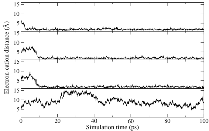
Figure 3: Electron-cation distance as a function of simulation time during unconstrained simulations of \text{Na}^+ and an excess electron with 300 water molecules, starting from 4 different initial configurations. Data obtained using the optimized set of parameters for the electron/sodium pseudopotential.
