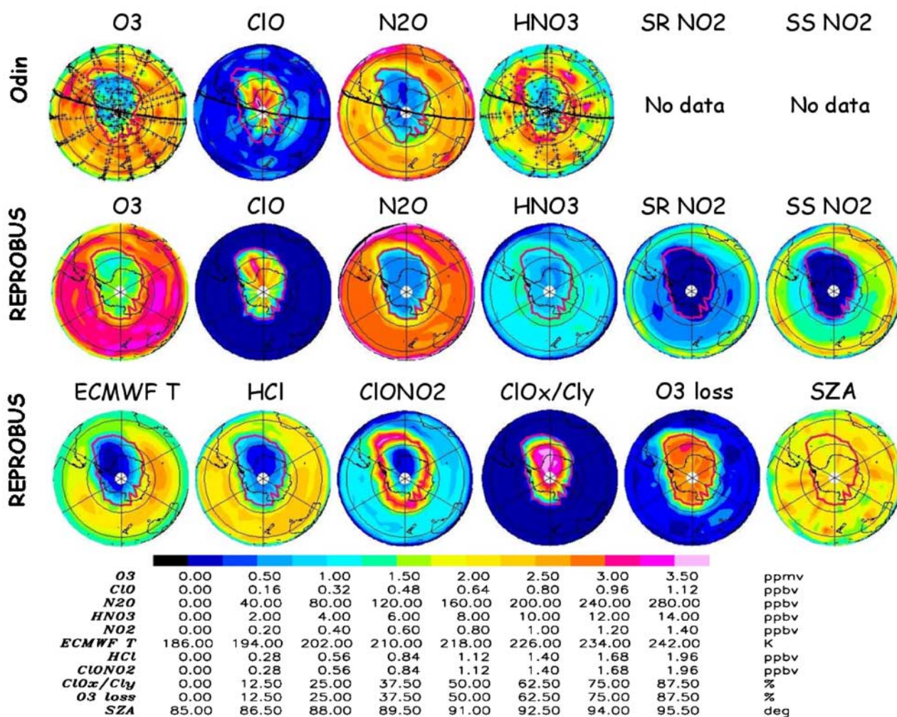
Figure 1. (top) From left to right, O 3 , ClO, N 2 O, and HNO 3 fields measured by Odin/SMR on 19–20 September 2002, interpolated onto the 500-K potential temperature surface. The maps are polar orthographic projections with black circles at 30°S and 60°S. Crosses represent the Odin orbit tracks over the 24-hour period starting from 1200 UT. Locations of ClO and N 2 O measurements are the same as O 3 and are not represented. The red line corresponds to the 120-ppbv N 2 O contour, which can be considered as the approximate edge of the polar vortex. The black line indicates the orbit track selected on Figure 2. Blank spaces represent data gaps or bad data points. Note that Odin measurements were performed at twilight (90° < SZA < 92.5°) on 19–20 September 2002 and during daytime (SZA ~85°) for the other days. (middle) From left to right, O 3 , ClO, N 2 O, HNO 3 , and sunrise (SR) and sunset (SS) NO 2 fields calculated by the REPROBUS chemical transport model on 19–20 September 2002, interpolated onto the 500-K potential temperature surface. Calculations are coincident in time and space with the Odin measurements. (bottom) From left to right, ECMWF temperature, HCl, ClONO 2 , ClO x /Cl y ratio, O 3 chemical loss calculated by REPROBUS (see text), and the solar zenith angle (SZA) at the time of the Odin measurements.
