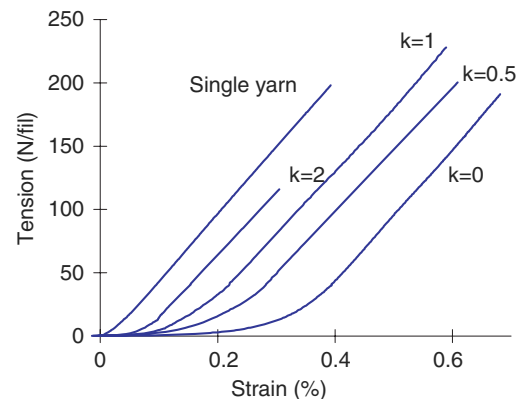
Fig. 5. Tension versus strain for different ratio k = \epsilon_{11}/\epsilon_{22} .
