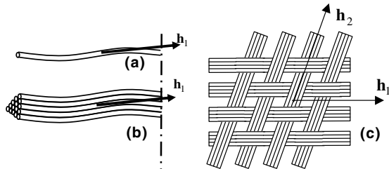
Fig. 1. (a) Single fibre, (b) yarn made of juxtaposed fibres, (c) woven yarns.
