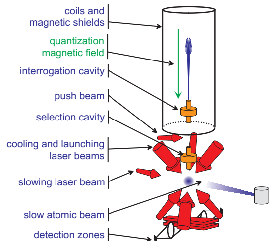
FIG. 1: Schematic view of an atomic fountain.
