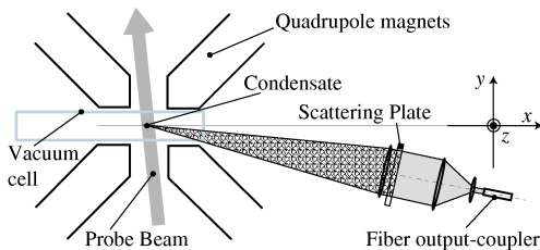
Figure 2: Optical setup used to create the random speckle potential. The BEC is at the focus of the lens system with its long axis oriented along the z direction.
