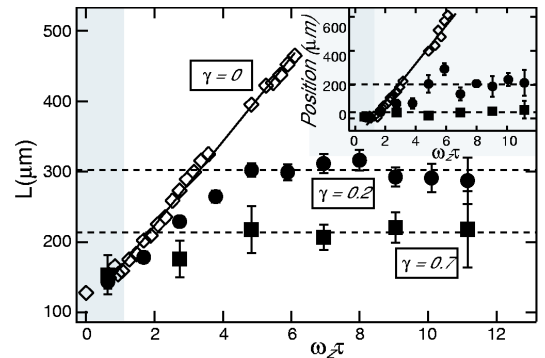
Figure 1: Time evolution of the axial rms size L of the BEC, for various amplitudes \sigma_V of the random potential, all smaller than the chemical potential \mu [ \gamma = \sigma_V/\mu = 0 ( \diamond ), 0.2 ( \bullet ) and 0.7 ( \blacksquare )]. The axial trapping frequency is initially \omega_z/2\pi = 6.7 Hz and is relaxed during the first 30 ms ( \omega_z\tau < 1.26 ) of the expansion time (grey band). Each point corresponds to an average over three measurements; error bars represent one standard deviation. The solid lines are linear fits to the data and the dashed lines are guides to the eye. Inset: Motion of the center of mass of the BEC during axial expansion for the same values of \gamma . Both sets of data show a strong suppression of transport of the BEC in the presence of disorder.
