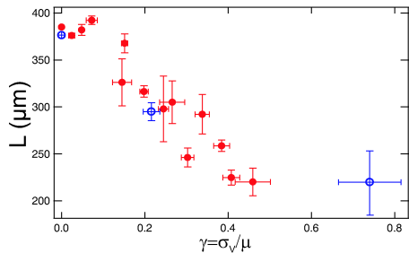
Figure 3: Rms size L of the BEC versus \gamma after an axial expansion time \omega_z \tau = 4.84 ( \tau = 115 ms). The open circles correspond to the curves of Fig. 1.
