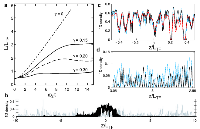
Figure 4: a) Time evolution of the rms size L of the BEC in the random potential V(z) for various values of the speckle amplitude \sigma_V = \gamma\mu as obtained from the numerical calculations. b) Density profile (black) and random potential V(z)/g_{1D} (gray) for \gamma = 0.2 at \omega_z \tau = 10 . c-d) Enlargement of density profile at \omega_z \tau = 10 (black solid) and \omega_z \tau = 20 (blue dotted). The red dashed line in c) is the Thomas-Fermi prediction (see text).
