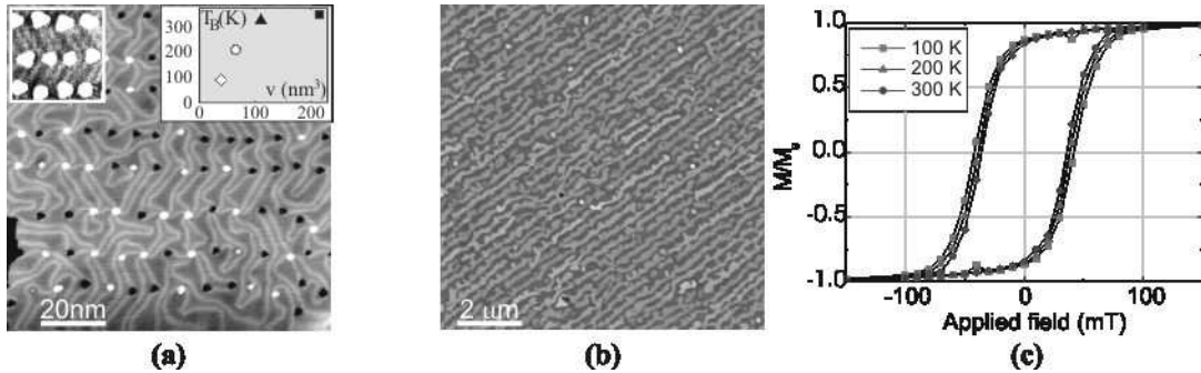
Figure 4. (a) STM image of a SO Co/Au(111) system during the fabrication of pillars. Insets: Conventional SO Co/Au(111) dots in the sub-AL range (left) and blocking temperature of pillars as a function of their volume [50] (right) (b) SO Fe/W/Mo(110) stripes, 4.3 nm-thick [95] (c) magnetization loops of Fe/W(110), 5.5 nm-thick, along in-plane [001].
