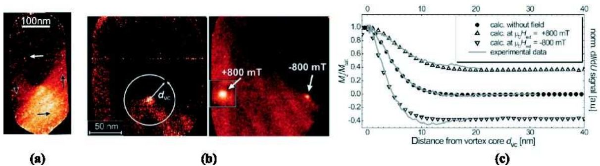
Figure 3. Micromagnetism with Sp-STM using an Fe/W(110) dot [77]. (a) overview of the flux-closure domain state, in-plane surface magnetization (b) out-of-plane component for zero-field (left), and in-perpendicular-field (right, main for negative field, inset for positive field). (c) surface profile of the vortex core.
