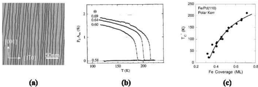
Figure 1. (a) differentiated STM image of SO Fe/W(110) stripes with 0.5 AL coverage [31] (b) in-plane remanent magnetization revealing a dramatic rise of apparent T_C (in reality, T_B , see text) upon percolation of SA Fe/W(110) dots around 0.6 AL (c) finite-size scaling for SO Fe/Pd(110) stripes. The line is a fit with Eq. (1) [32].
