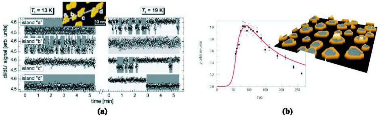
Figure 2. (a) spontaneous magnetization switching of SA Fe/Mo(110) dots (see inset) close to T_B , measured with Sp-STM [46] (b) T_B of SA Co rings fabricated around Pt(111) dots (inset) determined with susceptibility measurements [44]
