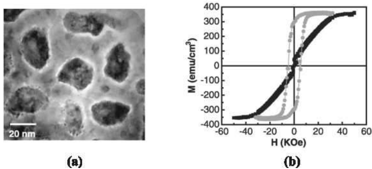
Figure 5. SO ferrimagnetic CoFe 2 O 4 columns in a BaTiO 3 ferroelectric matrix. (a) plane view (b) magnetization loops performed at 300 K for perpendicular (shaded) and in-plane (dark) field [9].
