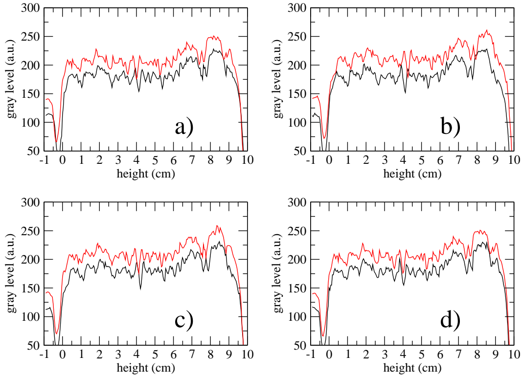
FIG. 5: Gray level profiles along a vertical line on the picture of the system for \Gamma = 2.4 : a) before (down) and after the first tap (up), b) just before the medium take off (down) and at its higher position (up), c) at its higher position (down) and just after the medium lands (up), d) just before (down) and after (up) the compression wave. For clarity, each curve has an offset in the y-axis and is reported in the reference frame of the vessel.
