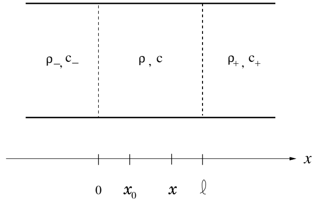
FIG. 1. 1D medium bounded with two other media.
