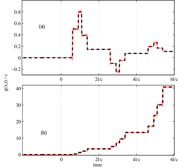
FIG. 2. Normalized Green function as a function of time: comparison between the successive reflections method (dotted line) and modal expansion (solid line, 102 modes, i.e. maximum n = 50 ). Locations of the source and receiver are x_0/\ell = 0.15 and x/\ell = 0.76 , respectively. (a) passive boundaries \zeta = 4 ; \zeta_\ell = 0.1 (constant mode = 0.097). (b) active boundary \zeta = \zeta_\ell = -4 . (constant mode = -2).
