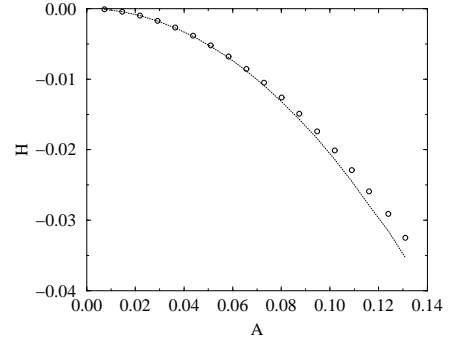
FIG. 13: Offset H of the equivalent boundary from the geometrical average of a self-affine profile of variable amplitude A , a roughness exponent \zeta = 0.8 and 16 modes. The dotted line is the result of the perturbation analysis, Eq.(49) and the symbols are the results obtained from a conformal mapping.
