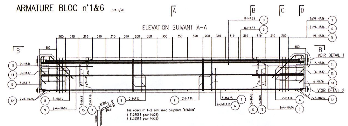
figure 2 Plan de ferrailage.
