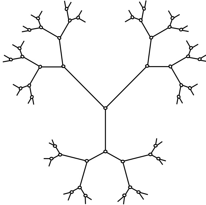
Figure 4 : Bruhat-Tits building of GL_2(K) , when |\kappa| = 2 .
