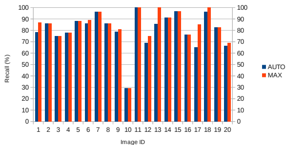
Figure 8: This figure shows the maximum recall obtained manually (MAX) and the adaptive segmentation (AUTO) for a sample of images of the dataset. Image 10 contains more than 60% of bright text over dark background which is not detected by our algorithm.
