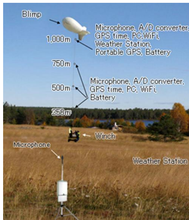
Figure 7: Outdoor measurement systems.
