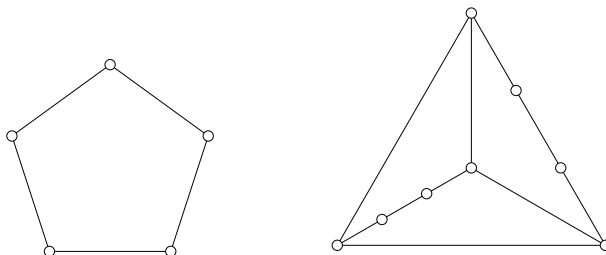
Figure 1: Dangerous graphs.
