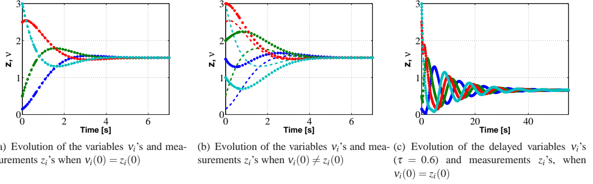
Fig. 3. Evolution of the additional dynamics v (dashed line) and the measurement vector z ( star line).
