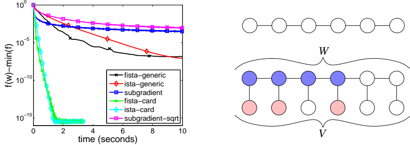
Figure 5: Left: Matlab running times of different optimization methods on 20 replications of a least-squares regression problem with p = 1000 for a cardinality-based submodular function (best seen in color). Proximal methods with the generic algorithm (using the minimum-norm-point algorithm) are faster than subgradient descent (with two schedules for the learning rate, 1/t or 1/\sqrt{t} ). Using the dedicated algorithm (which is not available in all situations) is significantly faster. Right: Examples of graphs (top: chain graph, bottom: hidden chain graph, with sets W and V and examples of a set A in light red, and B in blue, see text for details).
