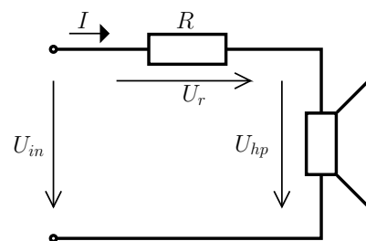
Figure 1: Impedance measurement of a loudspeaker using a shunt resistor.
