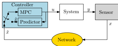
Fig. 8. Illustration of split sensing and control approach. The sensor transmits measurements asynchronously to save communication energy. The MPC controller uses local predictions when no measurement is received.
