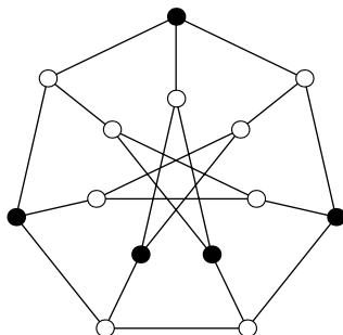
Figure 1: The generalised Petersen graph P(7, 2) has fourteen vertices and independence number 5. The black vertices form a maximum independent set.
