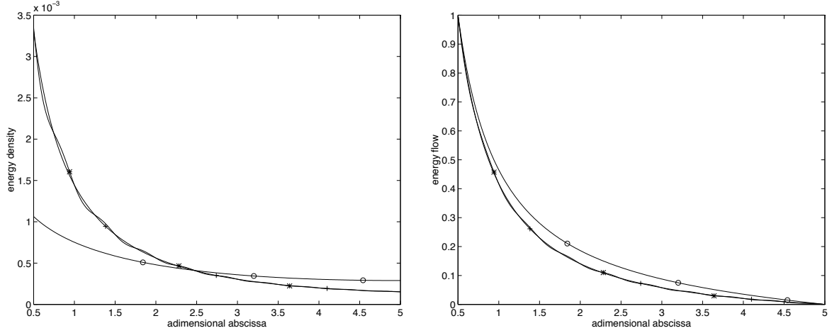
Figure 2: Comparison of energy densities and energy flows evaluated with three different methods for an axisymmetric membrane. *, equation of motion - o, diffusion equation (4) - +, energy equation (18).
