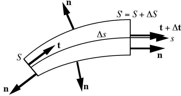
Figure 1: Geometric interpretation of the factor \Gamma .
