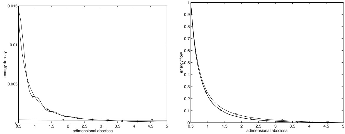
Figure 4: Comparison of energy densities and energy flows evaluated with three different methods for a spherical acoustical enclosure. *, equation of motion - o, diffusion equation (4) - +, energy equation (18).
