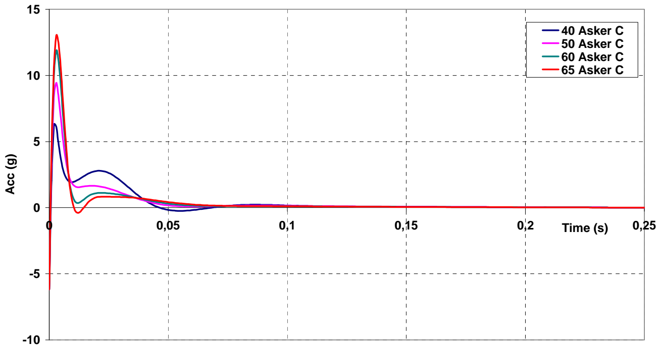
Figure 10 Acceleration of the mass m_1 [g] for soil S6 (ground stiffness k_s = 880 kN/m); load frequency 1.5 Hz.
