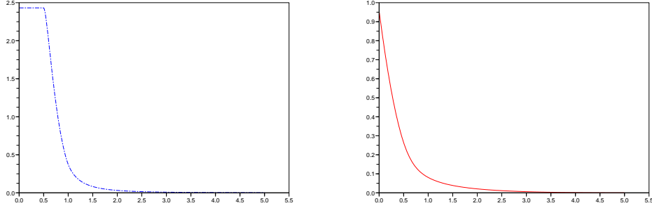
FIGURE 13. Graph of \Phi(t) (right) and g(t) = \Phi''(t) (left)
