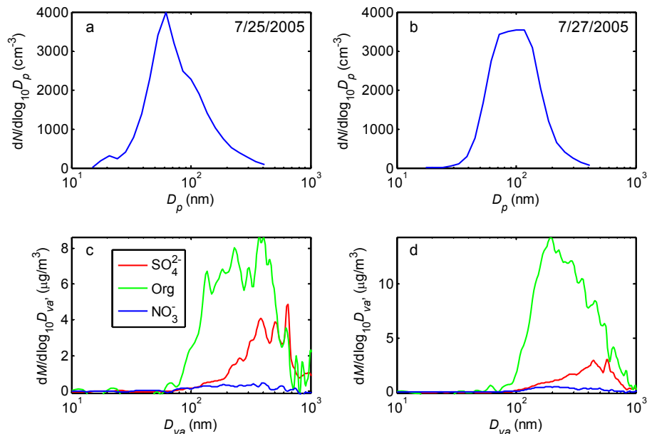
Fig. 4. Aerosol number size distribution ( a and b ) and mass size distributions of SO 4 2- , organics, and NO 3 - ( c and d ) for aerosols observed in thin layers above clouds on 25 July 2005 (a and c) and 27 July 2005 (b and d).
