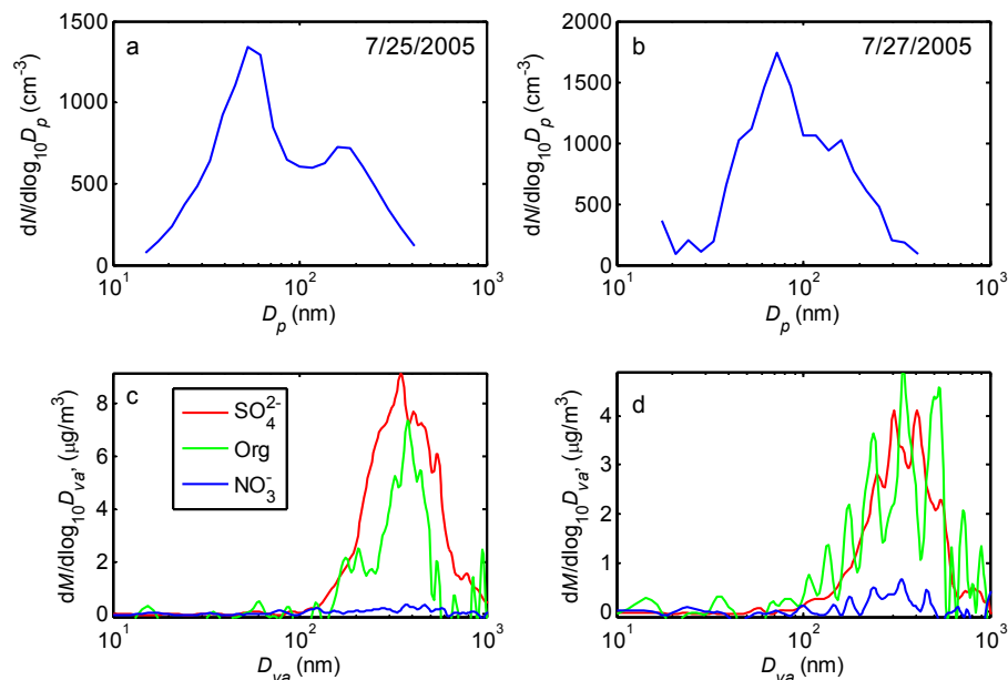
Fig. 3. Aerosol number size distribution ( a and b ) and mass size distributions of SO 4 2- , organics, and NO 3 - ( c and d ) for aerosols observed in boundary layer over ocean on 25 July 2005 (a and c) and 27 July 2005 (b and d).
