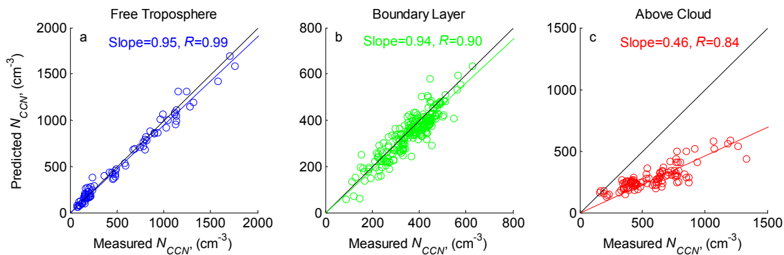
Fig. 6. Comparison of predicted and measured CCN at 0.22% for (a) Free Troposphere, (b) Boundary layer, and (c) Above Cloud aerosols.
