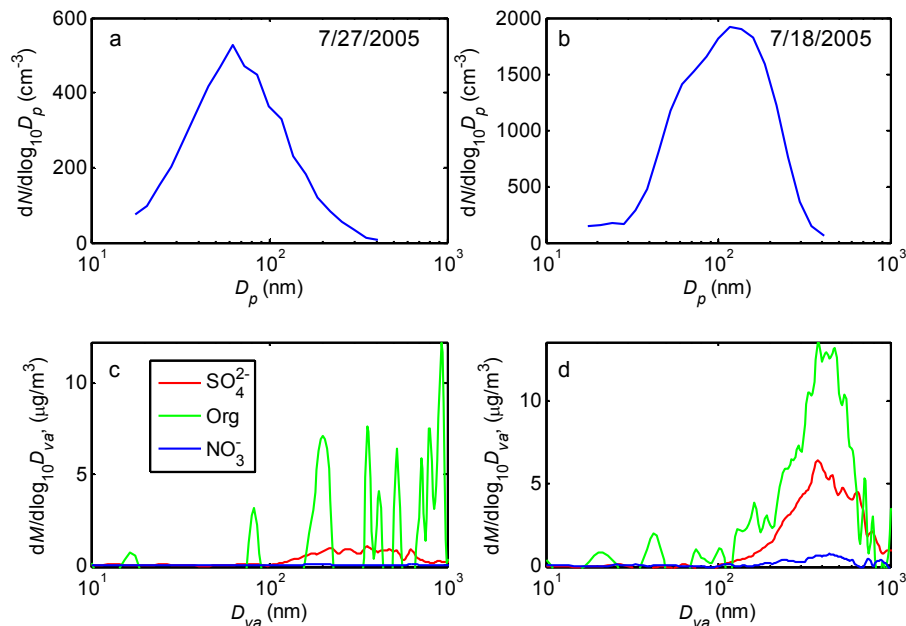
Fig. 2. Aerosol number size distribution ( a and b ) and mass size distributions of \text{SO}_4^{2-} , organics, and \text{NO}_3^- ( c and d ) for aerosols observed during ferry flights on 27 July 2005 ( a and c ) and 18 July 2005 ( b and d ).
