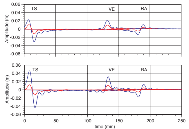
Fig. 9. Synthetic mareograms for Zone 6, magnitude, M=7.0 . Above: dip angle= 45^\circ ; below: dip angle= 30^\circ . Blue line, d=20 km; red line, d=40 km.
