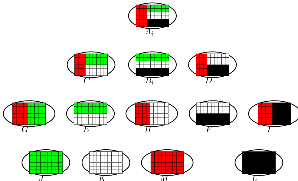
Figure 3: Cantor-Bendixson ranks
