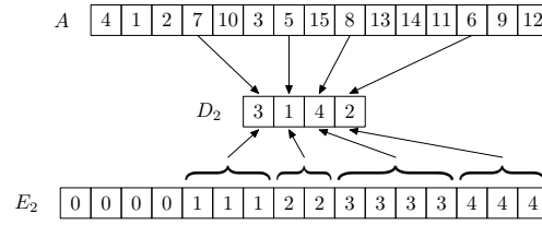
Figure 2: Example of computing arrays D_j and E_j , for n = 15 , \varphi = 4 , j = 2 , K_j = [5..8]
