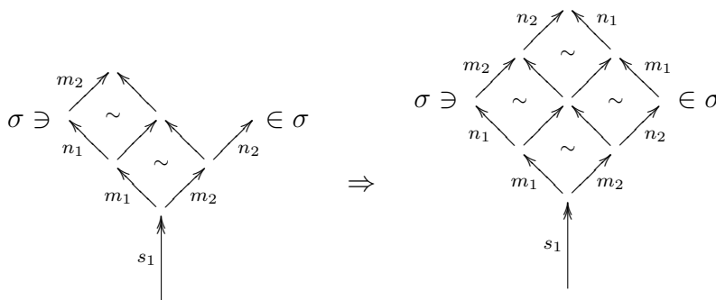
Fig. 2. Forward consistency
