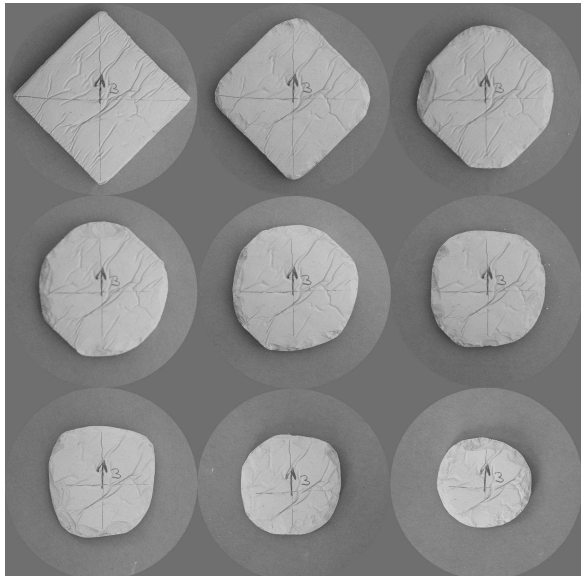
FIG. 3: Shape evolution of a 5 \times 5 \text{ cm} square pebble eroded in the laboratory, by the method explained in the text. The images were taken at 5 min intervals, and are shown at the same magnification.
