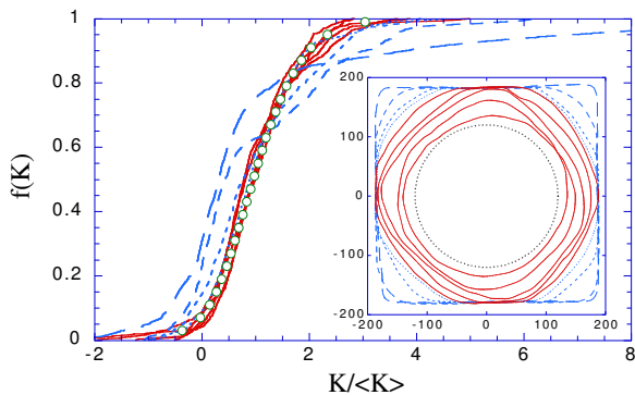
FIG. 4: (Color online) Cumulative curvature distribution, f(K) , for the evolving pebble depicted in the inset (and pictured in Fig. 3). As the pebble becomes progressively rounder, the curvature distribution narrows and approaches a final shape. The time interval between successive contours is 5 minutes; the early contours of evolving shapes are shown as different blue dashes, while the later contours of stationary shape are shown as solid red. The same color and curve types are used in the main plot. For the inset, the axes are given in pixel units, equal to 0.132 mm. For contrast, a circle is shown by points.
