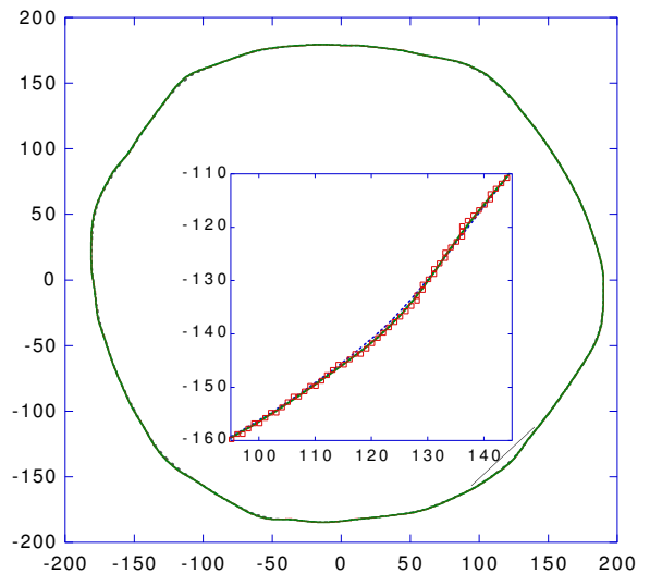
FIG. 10: (Color online) Reconstruction of a smooth pebble contour from the pixelized digital representation. The solid curve is based on fitting to cubic polynomials at each point. The dashed curve is based on the iteration scheme of Fig. 11.
