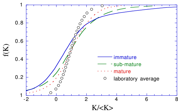
FIG. 9: (Color online) Cumulative curvature distribution, f(K) , for the average shapes of Mont St.-Michel rip-up clasts. Even the roundest shapes remained less circular than the final shape in the laboratory study.
