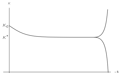
Figure 2.13: Behavior of \kappa(k) very close to \kappa_c .
