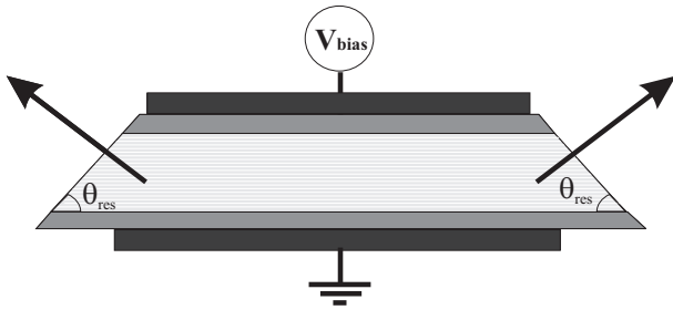
FIG. 6: Sketch of a possible set-up for the generation of correlated photon pairs in the intersubband cavity system. The vacuum Rabi frequency of the intersubband cavity system can be modulated through an electric gate, which changes the density of the two-dimensional electron gas or alternatively the dipole moment of the intersubband transition. A modulation of the bias is expected to induce the emission of correlated photon pairs with opposite in-plane wavevectors. This kind of radiation can be optimally guided out of the cavity through wedged lateral facets, with inclination equal to the resonance angle \theta_{res} .
