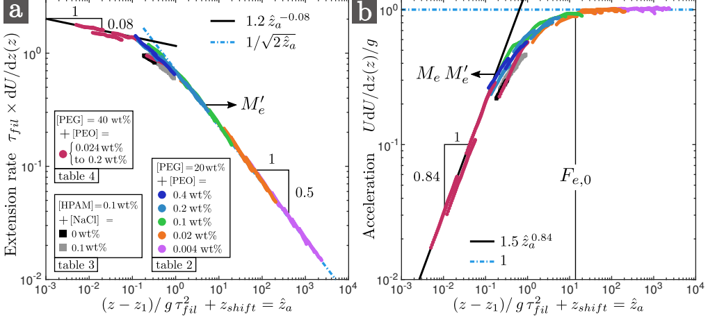
FIGURE 21. (a) Dimensionless extension rate \tau_{fil} dU/dz(z) and (b) dimensionless acceleration U dU/dz(z)/g versus (z - z_1)/z_e + z_{shift} for the curtains of figure 20. The master curve M_e reaches the asymptotic free-fall regime at z/z_e about F_{e,0} = 12 \pm 5 since M_e M'_e(F_{e,0}) = 0.95 , where 0.95 is an arbitrary value close to 1.
