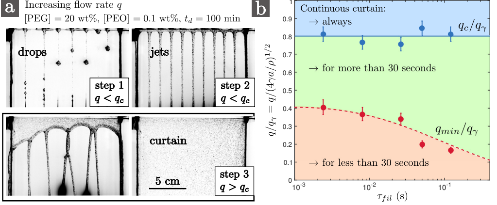
FIGURE 26. (a): Different regimes observed when increasing the flow rate from 0 to 6 \text{ cm}^2/\text{s} for the degraded ( t_d = 100 min) 0.1 wt% PEO solution with 20 wt% PEG solvent (table 2). (b): Critical flow rate q_c (above which any hole is advected by the flow) and minimum flow rate q_{min} (required to maintain a continuous curtain for more than 30 seconds), divided by q_\gamma = (4a\gamma/\rho)^{1/2} , against the extensional relaxation time \tau_{fil} for the five degraded ( t_d = 100 min) PEO solutions with 20 wt% PEG solvent (table 2). q_\gamma = 3.5 \text{ cm}^2/\text{s} and curtain length is L_c = 30 cm.
