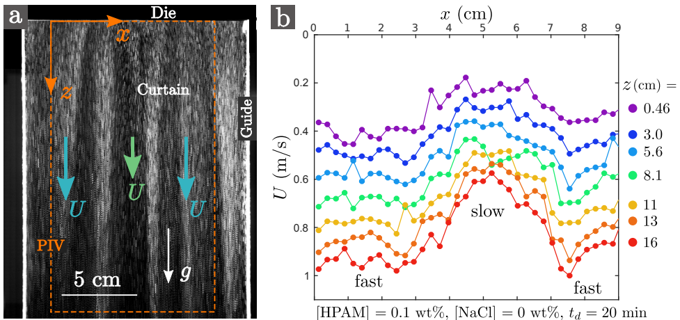
FIGURE 9. Example of PIV measurement for a degraded ( t_d = 20 \text{ min} ) 0.1 wt% unsalted HPAM solution (table 3). (a): Superposition of six successive PIV images. The correlation algorithm is applied to a domain restricted to the dashed rectangle. (b): z -component of the velocity field, i.e. U(x, z, t) , against the horizontal coordinate x at different distances z from the slot at an arbitrary time t . The curtain length is L_c = 30 \text{ cm} and the linear flow rate is q = 3.1 \text{ cm}^2/\text{s} .
