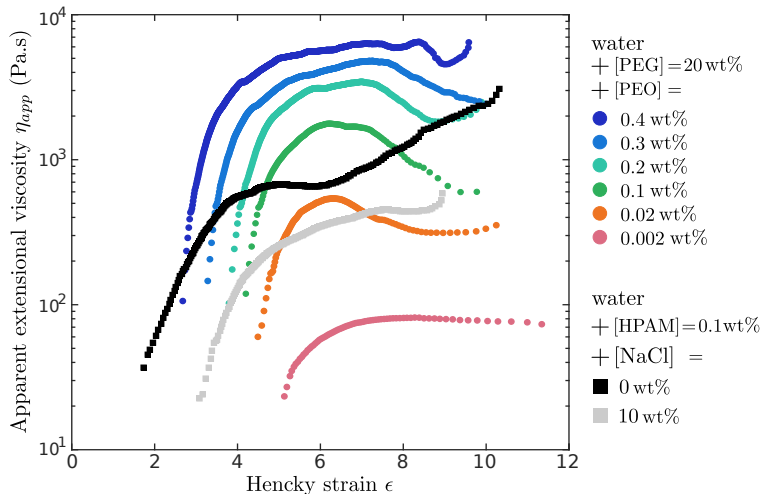
FIGURE 6. Apparent extensional viscosity \eta_{app} (equation 3.4) as a function of the Hencky strain \epsilon (equation 3.5) for PEO solutions with 20 wt% PEG solvent and for HPAM solutions at T = 20^\circ\text{C} .
