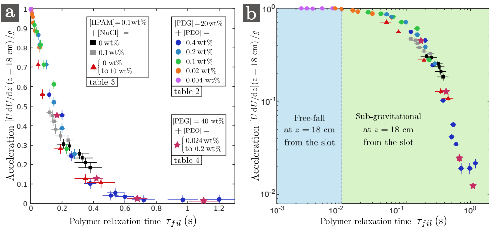
FIGURE 14. Dimensionless acceleration [UdU/dz]/g at z = 18 cm from the slot against polymer extensional relaxation time \tau_{fil} in lin-lin (a) and log-log (b) scales for all the solutions of tables 2 (PEO) and 3 (HPAM), for which the curtain length is always L_c = 30 cm, and for all PEO the solutions of tables 4 when the curtain length is also L_c = 30 cm. Note that another 0.4 wt% PEO solution with 20 wt% PEG solvent was prepared and that the curtain flow was measured at t_d = 0, 5, 10 , and 20 minutes in order to fill the high relaxation time region of the curve.
