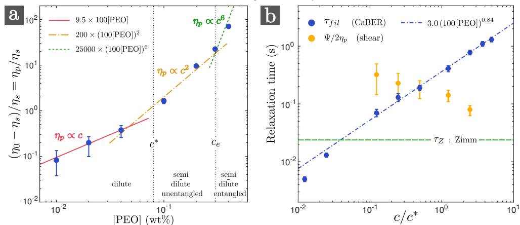
FIGURE 27. Some data for the PEO solutions with 20 wt% PEG solvent of table 1. (a) Evolution of the polymer contribution to the zero-shear viscosity \eta_p = \eta_0 - \eta_s (divided by the solvent viscosity \eta_s ) with polymer concentration [PEO] . (b): Comparison of the different relaxation time estimations: \Psi/2\eta_p (shear measurements for quadratic normal stress differences N_1 = \Psi\dot{\gamma}^2 ), \tau_{fil} (CaBER) and \tau_Z = 0.024 s (Zimm theory, equation A 1) against dimensionless polymer concentration c/c^* where c = \rho [PEO] and where c^* = 0.83 kg/m 3 is the critical overlap concentration.
