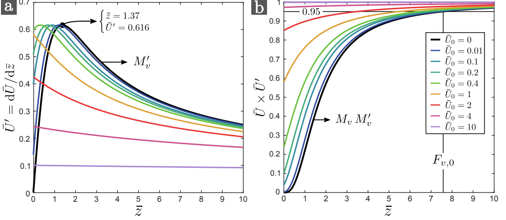
FIGURE 19. Dimensionless extension rate \bar{U}'(\bar{z}) (a) and acceleration \bar{U}\bar{U}'(\bar{z}) (b) for an infinitely long curtain made of a Newtonian liquid (equation 5.4 for C = 0 ), starting from various initial velocities \bar{U}_0 ranging between 0 and 10. The master curve M_v has an inflection point at \bar{z} \approx 1.37 , where the elongation rate reaches a maximum value M'_v(1.37) \approx 0.616 , and reaches the asymptotic free-fall regime at \bar{z} = F_{v,0} \approx 7.56 since M_v M'_v(F_{v,0}) = 0.95 , where 0.95 is an arbitrary value close to 1.
