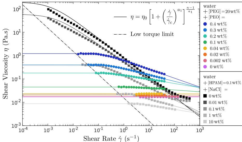
FIGURE 3. Apparent shear viscosity \eta(\dot{\gamma}) for PEO solutions with 20 wt% PEG solvent and for HPAM solutions at T = 20^\circ\text{C} . Data are fitted with a Carreau law (equation 3.1). The low-torque limit is shown.
