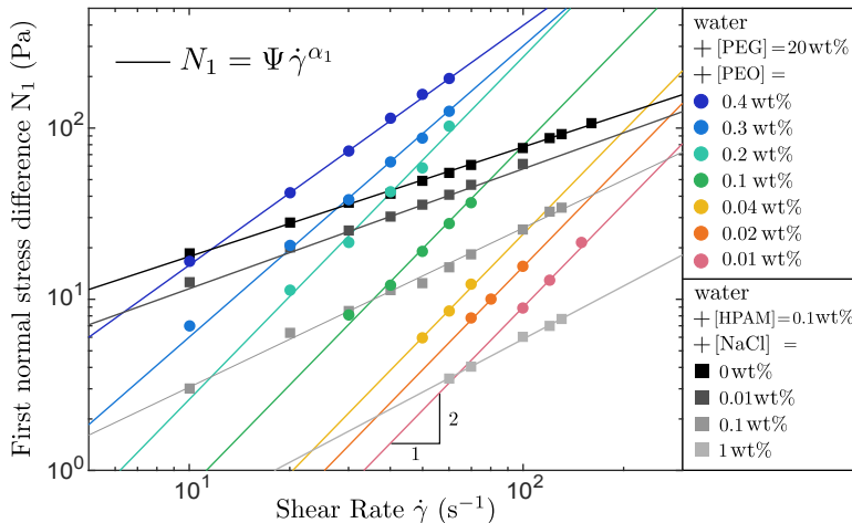
FIGURE 4. First normal stress difference N_1(\dot{\gamma}) for PEO solutions with 20 wt% PEG solvent and for HPAM solutions at T = 20^\circ\text{C} . Data are fitted with a power law (equation 3.2).
