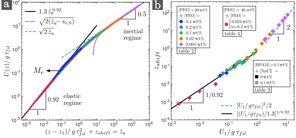
FIGURE 20. (a): Master curve of viscoelastic curtains. Dimensionless velocity field U(z)/g\tau_{fil} against (z - z_1)/g\tau_{fil}^2 + z_{shift} in log-log scale, where z_1 \approx 2.5 mm, and where each curve is translated by a distance z_{shift} in order to rescale all the data on a single curve. The master curve M_e is characterised by an initial (sub-gravitational) elastic regime and an asymptotic (free-fall) inertial regime (equation 5.23). (b): When plotting z_{shift} against U_1/g\tau_{fil} , we find that z_{shift} = M_e^{-1}(U_1/g\tau_{fil}) . We only consider the curtain flows which are presumably not influenced by the downstream boundary condition. For the PEO solutions with 40 wt% PEG solvent of table 4, we only take the longest curtains, for example L_c = 200 cm for the data of figure 11.a. Besides, for the PEO and HPAM solutions of tables 2 and 3 (top) which correspond to curtains of length L_c = 30 cm, we show the velocity profile for z < 20 cm only for the solutions with extensional relaxation times \tau_{fil} \leq 0.2 s since the experiments reported in §4.3 suggest that the effect of the downstream boundary condition is out of frame.
