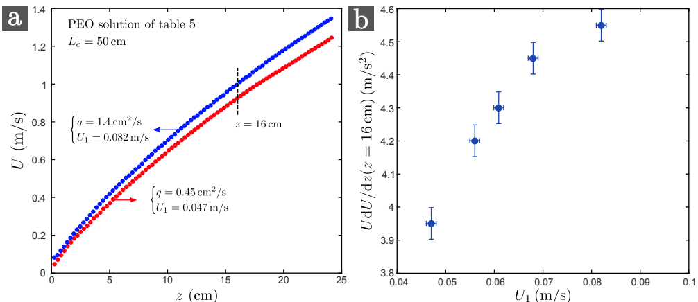
FIGURE 12. (a): Velocity field U(z) for the PEO solution of table 5 extruded at flow rates q = 0.45 cm 2 /s and 1.4 cm 2 /s. The liquid velocity U_1 at z_1 \approx 2.5 mm from the slot is respectively 0.047 m/s and 0.082 m/s. (b): Local acceleration UdU/dz at an arbitrary distance z = 16 cm from the slot versus initial velocity U_1 . The curtain length is L_c = 50 cm.
