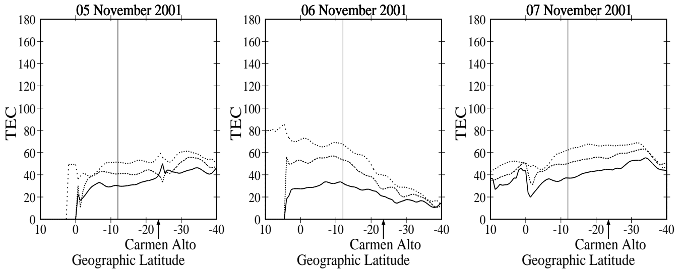
Fig. 10. Total electron content ( \times 10^6 electrons \text{cm}^{-2} ) along American longitude sector, derived from the GPS phase fluctuations for 5–7 November 2001, at 06:00 LT (solid line), 07:00 LT (middle line) and 08:00 LT (dotted line). During this time period, enhancements were observed in the dayglow emissions on 6 November (see Fig. 7). Magnetic equator is shown as a vertical line. Carmen Alto is located at approximately 23.16^\circ geographic latitude as indicated by an arrow. It can be seen that the TEC on 6 November did not show any increase corresponding to the increase in dayglow emissions. Actually, a factor of 1.5–2 smaller TEC was measured on this day compared with the quiet day, thus indicating no role of electron densities in the observed dayglow emission enhancement. Hence, it is suggested that a possible increase in the neutral densities be responsible for the rise in the observed dayglow emissions on this day. Also, the asymmetric nature of the TEC distribution with respect to latitude on 6 November indicates the presence of strong equatorward winds that bring neutrals from the high latitudes.
