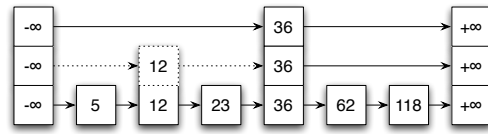
Figure 3: Adapting vertically the skip list structure
