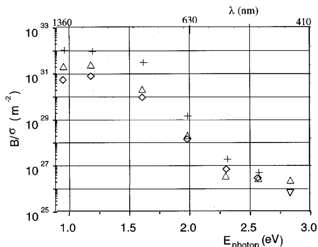
Fig. 6. Dependence of photostability FOM B/\sigma on photon energy for three guest chromophores in a PMMA host. The azodyes 5 (+), 6 (◇), and 7 (△) differ only by the site of attachment of a \text{CF}_3 group on the benzene rings in the common 4- N,N -diethylamino-4'-nitroazobenzene unit.
