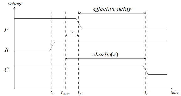
Fig. 6. Ring stage timing diagram
