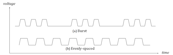
Fig. 5. Burst and evenly-spaced propagation modes in STRs
