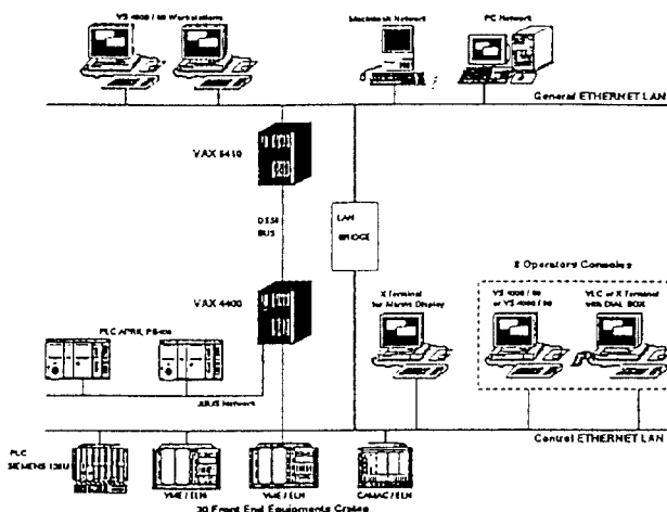
Figure 1 : The general control system layout
