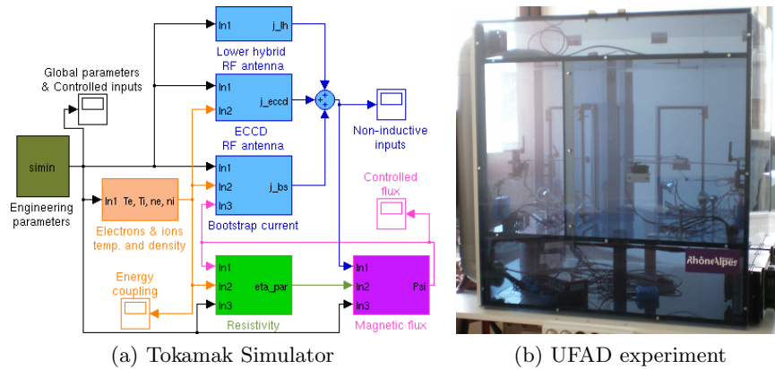
Fig. 1: Examples of PBL applications for green SCIT: sustainable power generation (tokamak) and intelligent buildings (UFAD).
