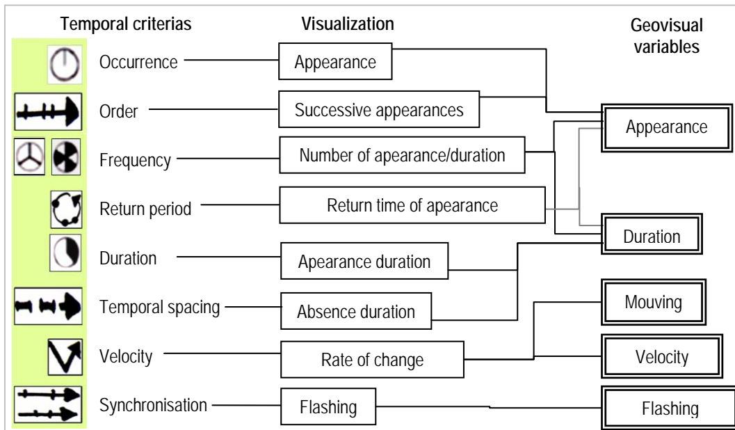
Figure 3: Geovisual variables
