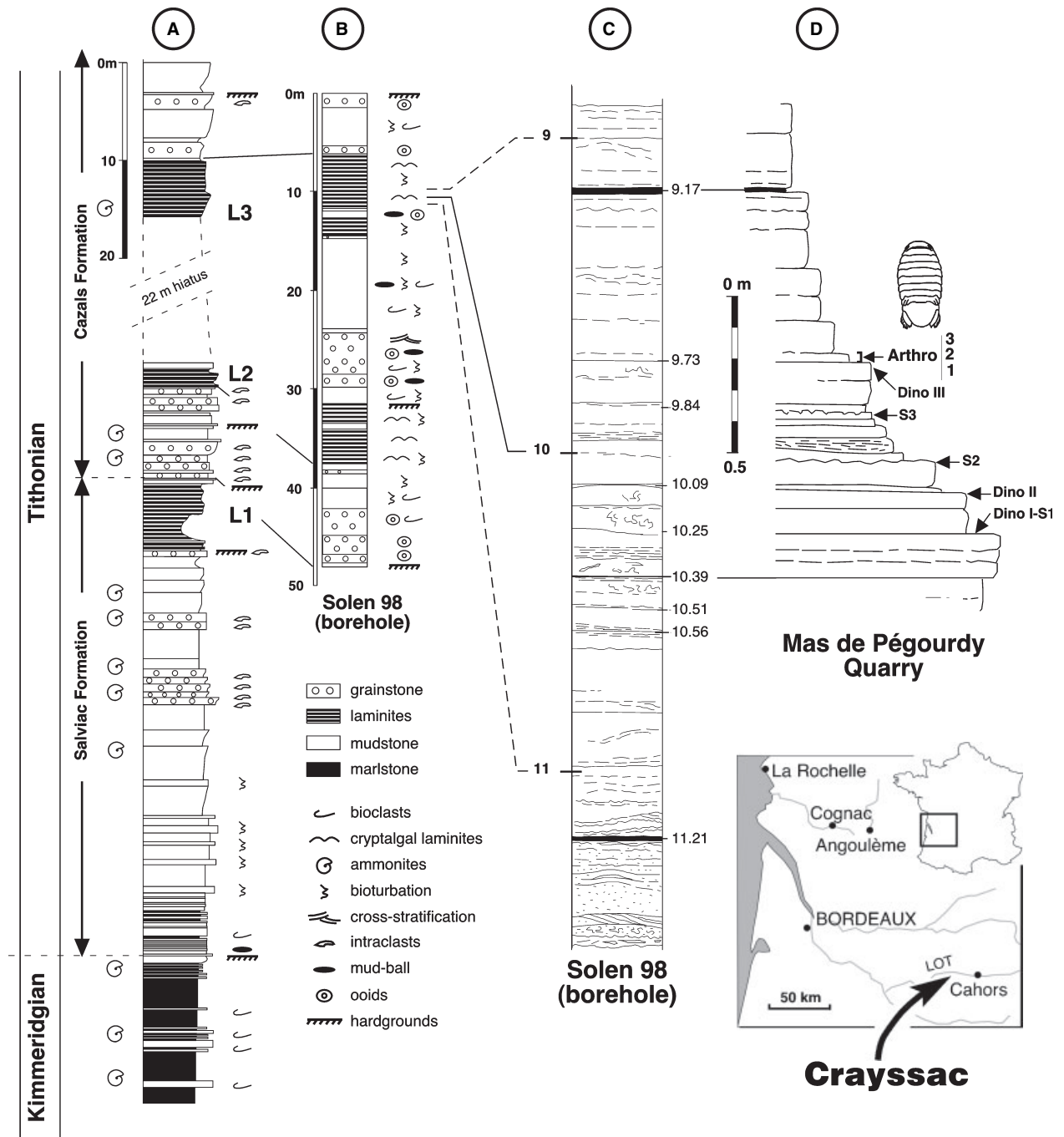
TEXT-FIG. 1. Lithology and stratigraphy of the Crayssac Fossil Lagerstätte. A, reconstructed lithological succession of the Upper Jurassic in the Quercy area (after Hantzpergue and Lafaurie 1994). B–C, Solen 98 drill core. D, occurrence of Pterichmus and other trackways in the Mas de Pégourdy quarry (Crayssac, Lot); Arthro 1–3, Pterichmus beds; Dino I–III, main surfaces with dinosaurs tracks.
