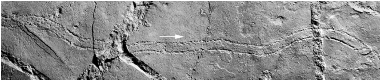
TEXT-FIG. 12. Pterichnus isopodicus sp. nov., long trackway interrupted at one end (either death mark or terminal animal burrow), Arthro 2 bed, Mas de Pégourdy quarry, field photograph; white arrow indicates the assumed direction of movement of the trace-maker; \times 0.5 .
