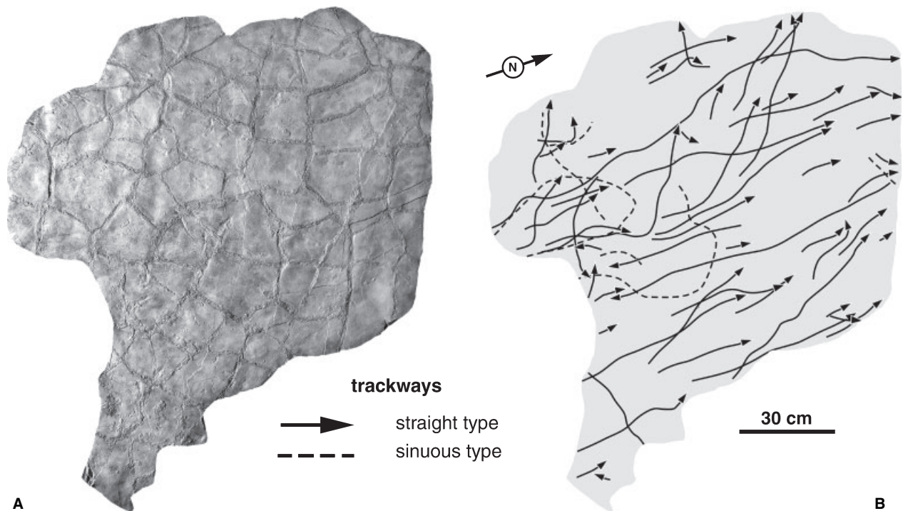
TEXT-FIG. 11. Numerical abundance and preferential orientation of Pterichmus isopodicus isp. nov. along Arthro 2 bed, same locality and age as in Text-fig. 4. A, resin replica from rock slab (FSL 525005) showing mudcrack network. B, trackway mapping from same slab with solid and dotted lines representing orientated (Types 1 and 2) and sinuous (Types 3 and 4) trackways, respectively (see text).
