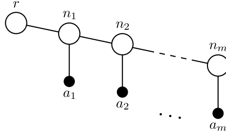
Figure 2: Instance \mathcal{I}_4 .
