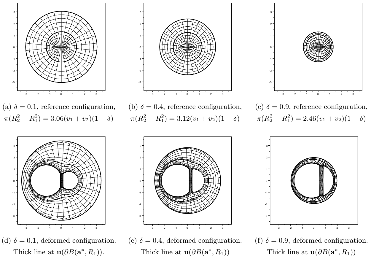
Figure 6: Transition to a radially symmetric map. A larger initial domain is necessary in order to create spherical cavities. Parameters: \Omega = B(\mathbf{0}, R_2) , \sqrt{\frac{v_1 + v_2}{\pi d^2}} = 1.5 , \frac{v_2}{v_1} = 0.3 , d = 1 , R_1 \approx d .
