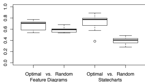
Figure 10. Comparison of the dissimilarity criteria measure, optimal solutions generated by our approach vs. random solutions for both metamodels
