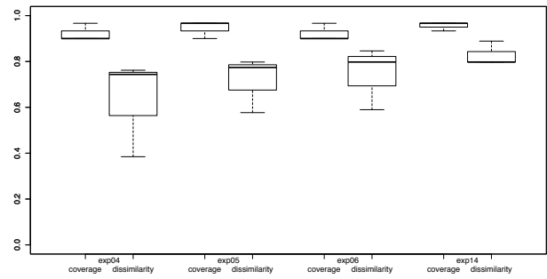
Figure 8. Coverage and dissimilarity measures for the statecharts metamodel
