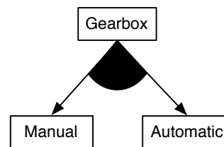
Figure 2. A feature diagram in the modeling language’s concrete syntax.
