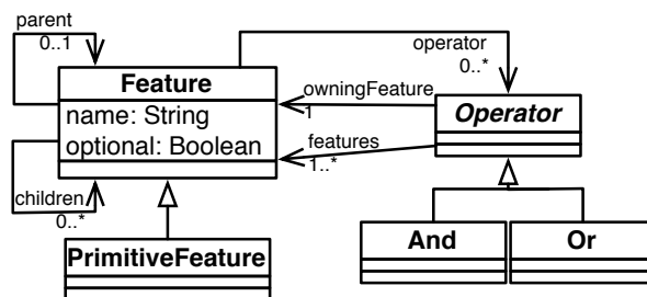
Figure 1. Metamodel for Feature Diagrams.
